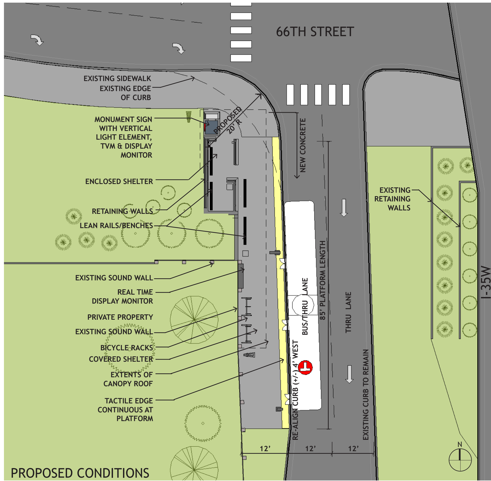
SOUTHBOUND CONCEPT D - FARSIDE
