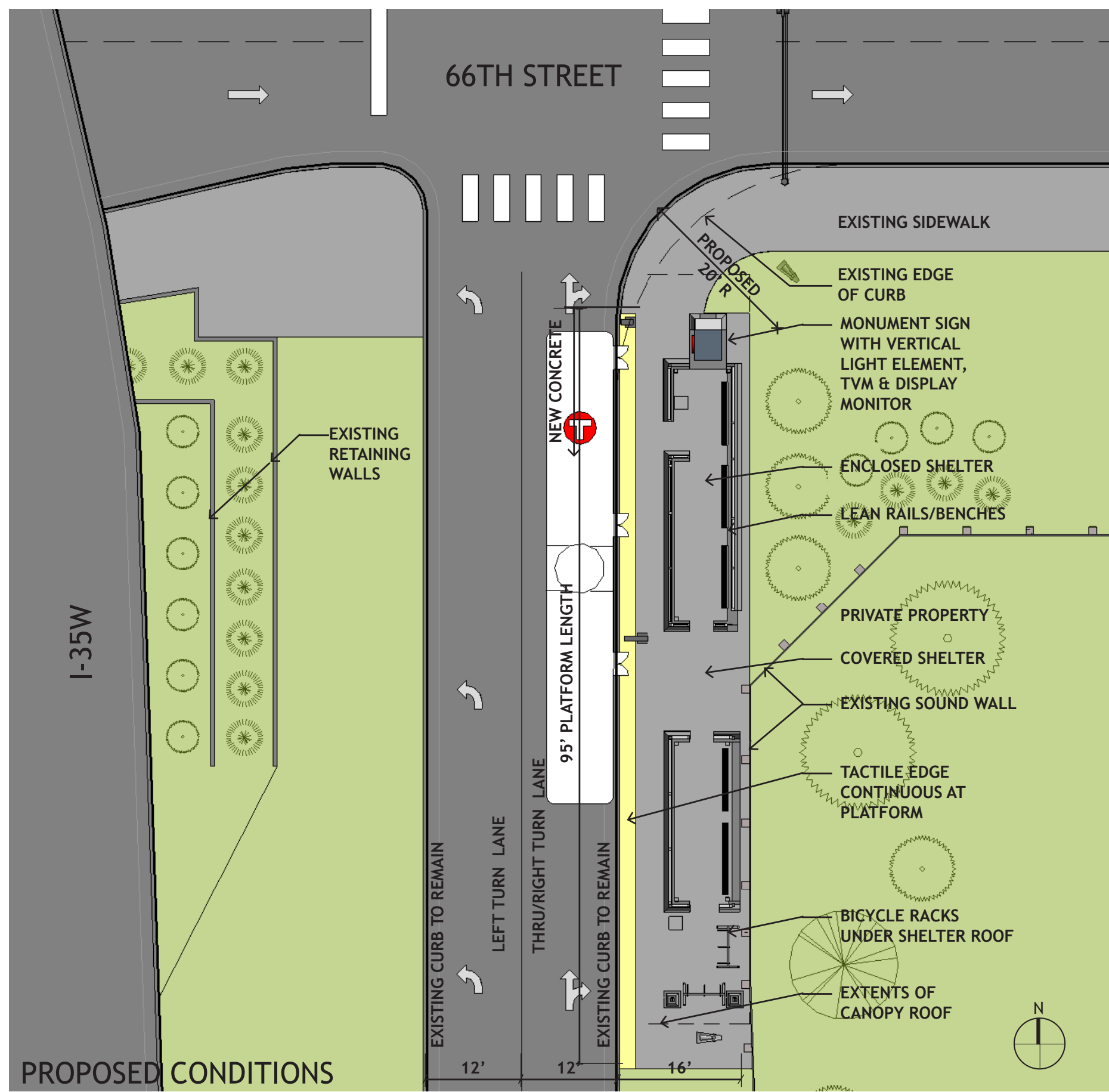
NORTHBOUND CONCEPT A - NEARSIDE
