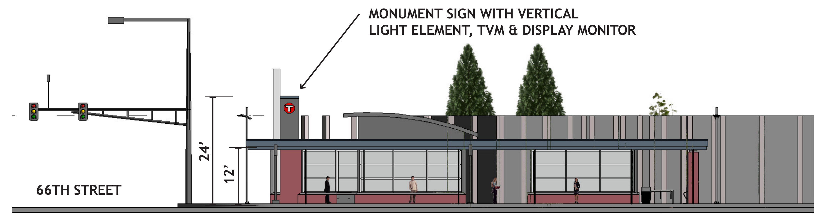
NORTHBOUND PLATFORM - ELEVATION LOOKING EAST
