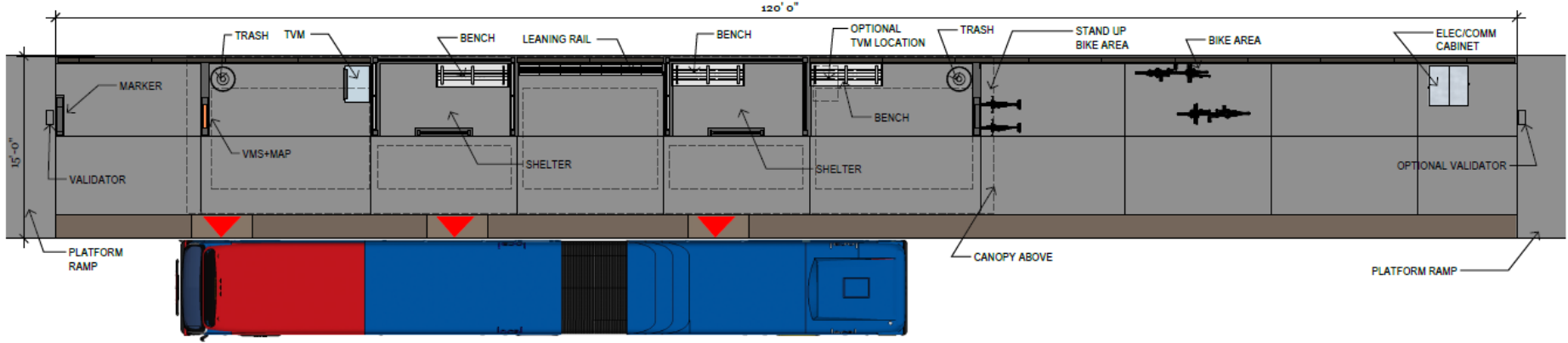
PLAN 1/8" = 1'-0"
