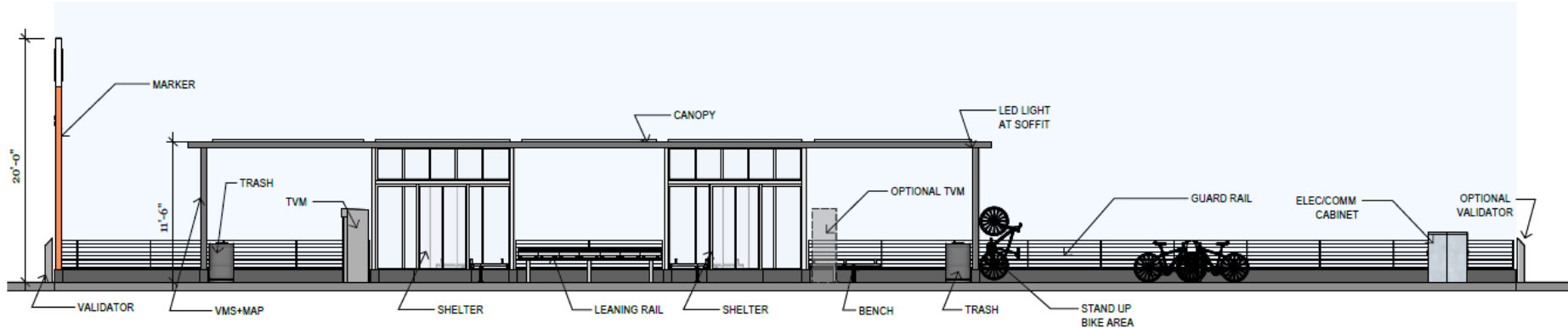
ELEVATION 1/8" = 1'-0"
