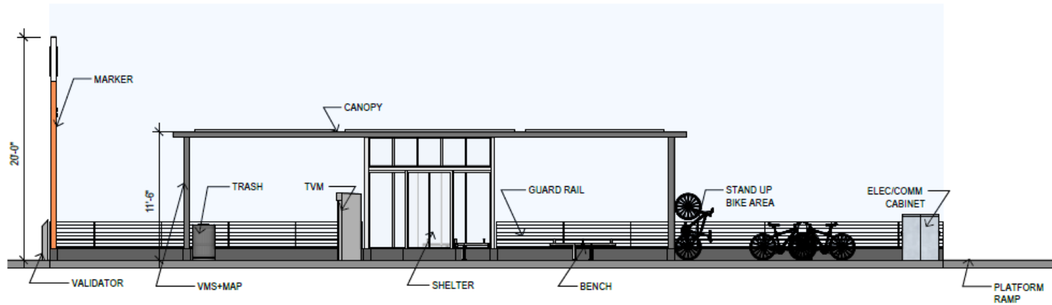
ELEVATION 1/8" = 1'-0"
