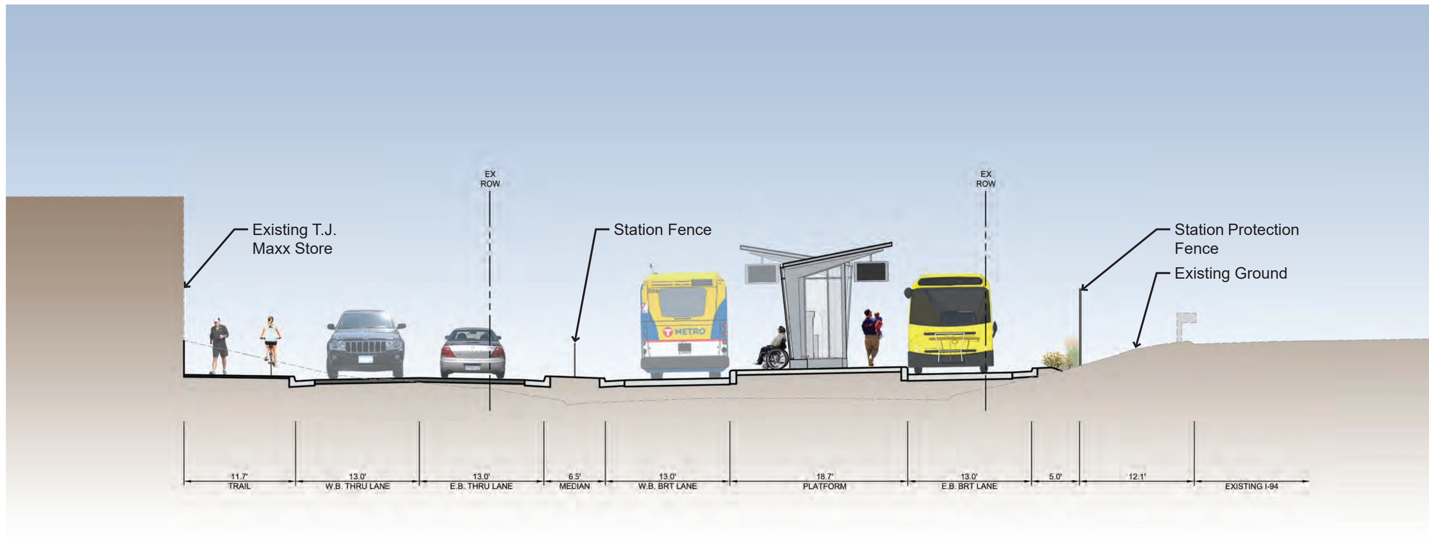
Section A-A: Looking East
