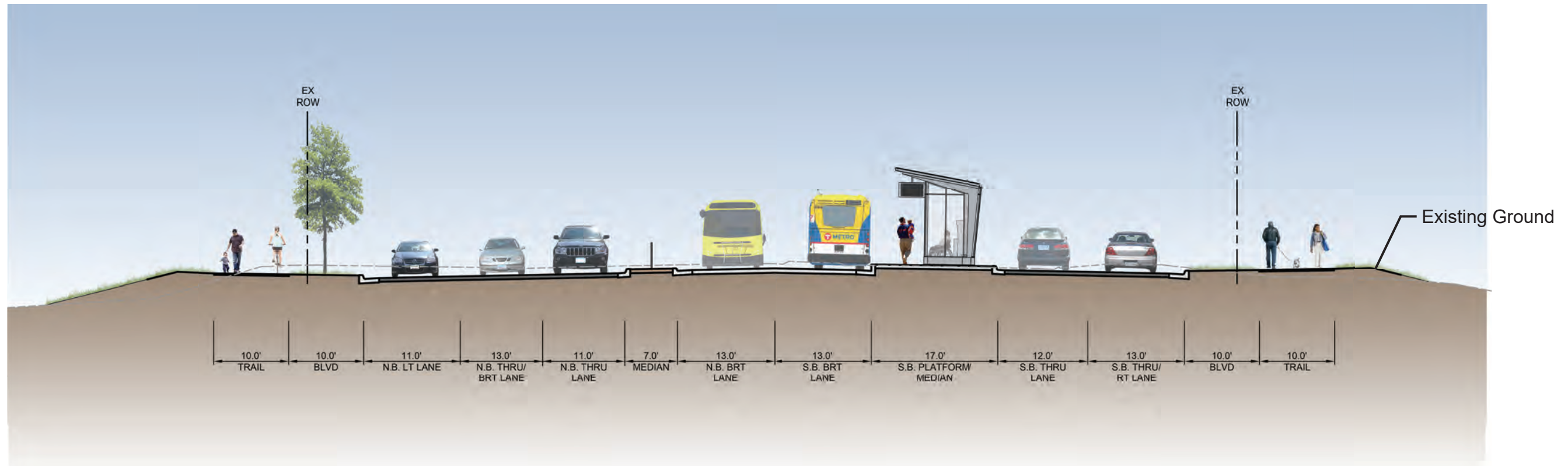
Section A-A (Looking South)
