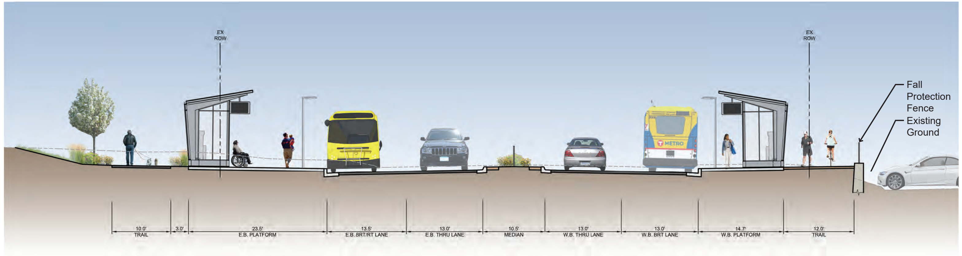
Section A-A (Looking West)
