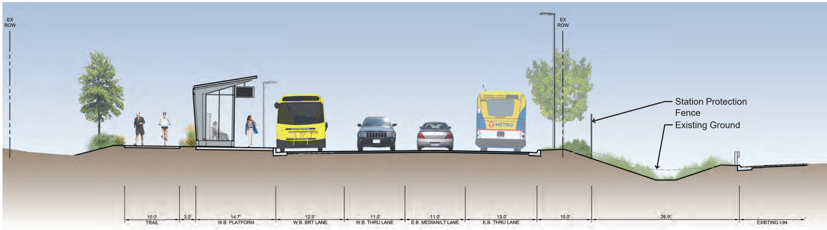
Section A-A: WB Platform (Looking East)
