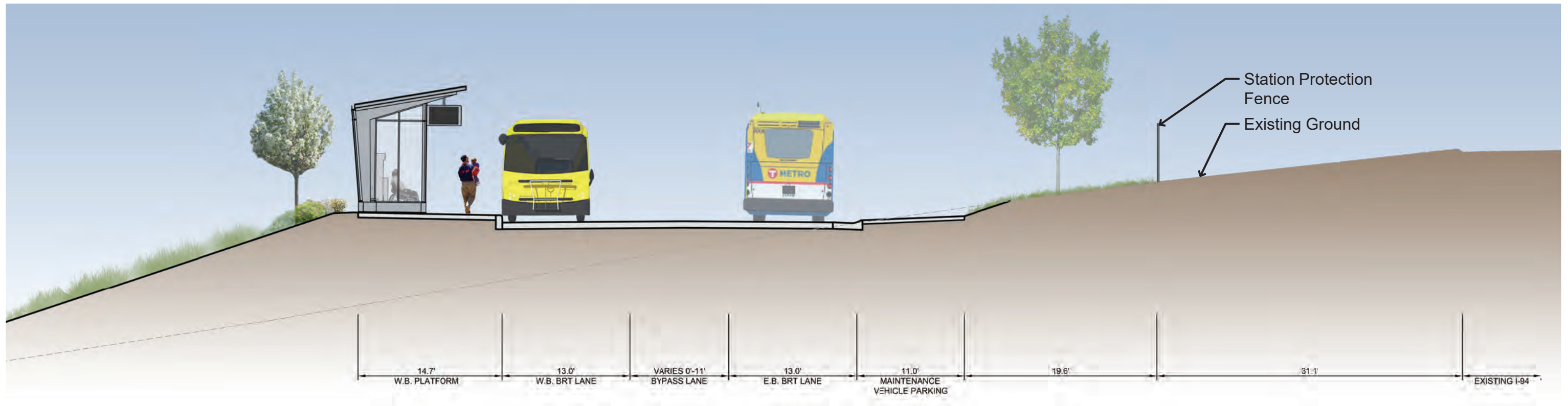
Section A-A: W.B. Platform (Looking East)
