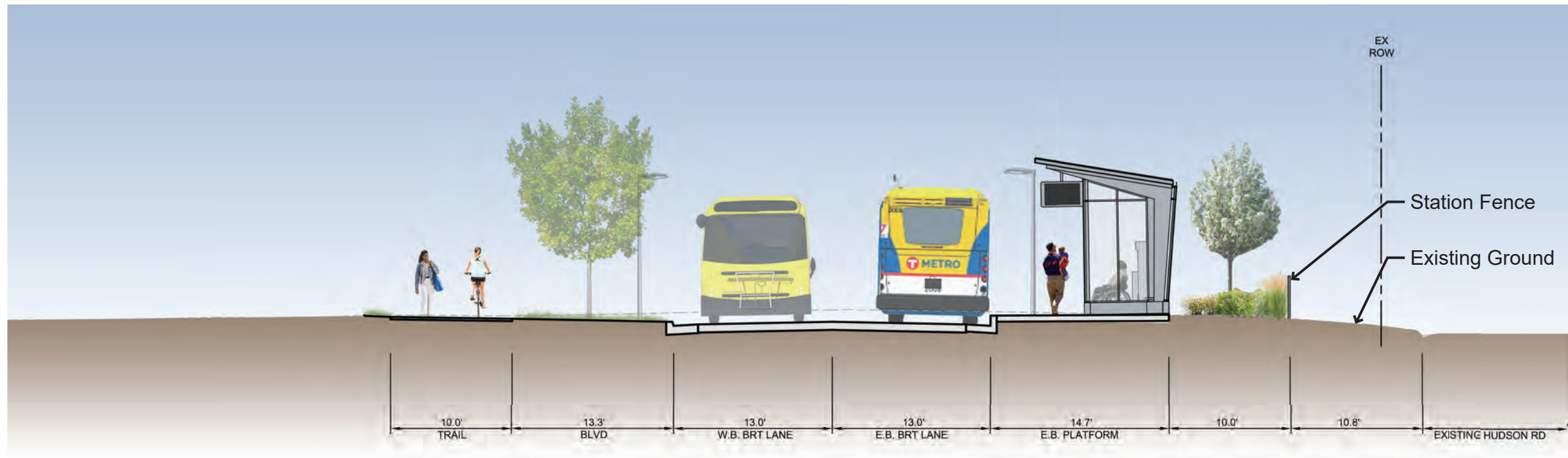
Section A-A: EB Platform (Looking East)
