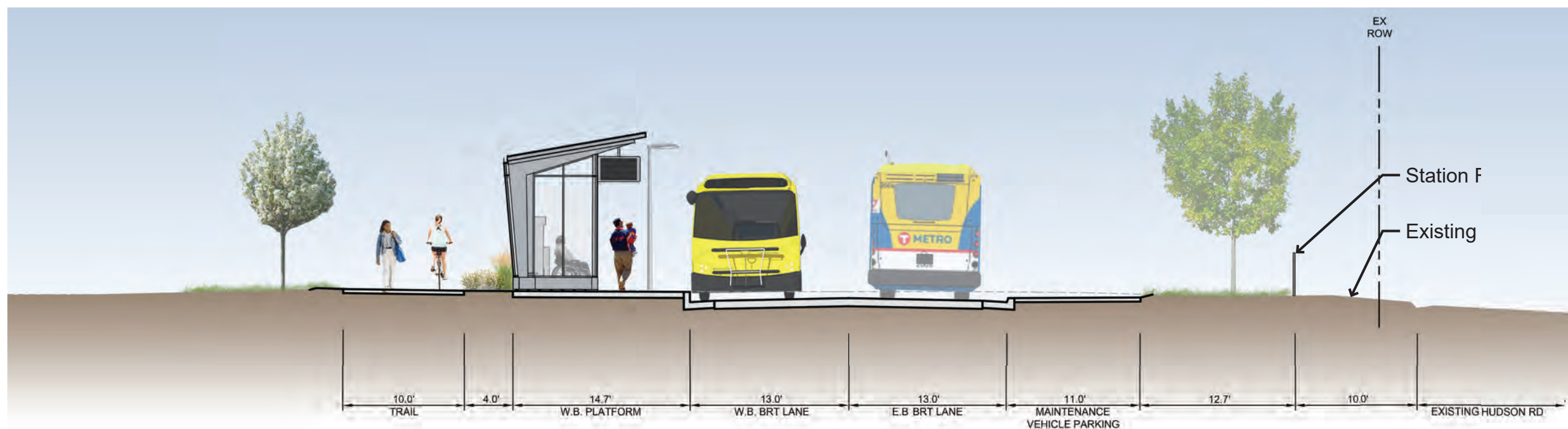
Section B-B: WB Platform (Looking East)
